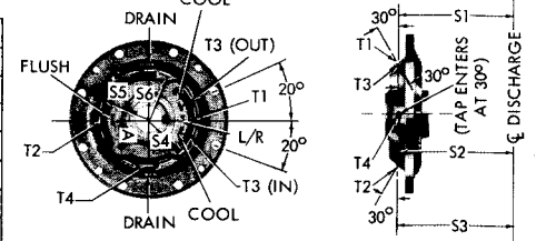
VIEW Z-Z
