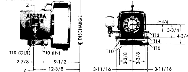
RECOMMENDED FOUNDATION:
