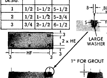
RECOMMENDED FOUNDATION:
