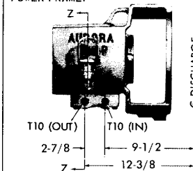
POWER FRAME:
