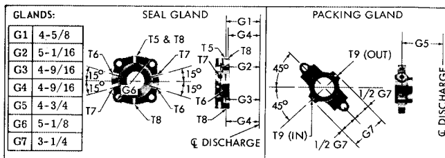
STUFFING BOX:
