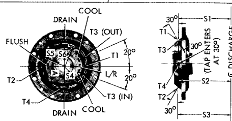
STUFFING BOX:
