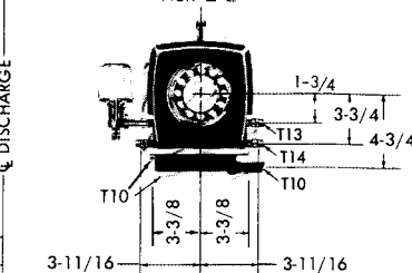
VIEW Z-Z
